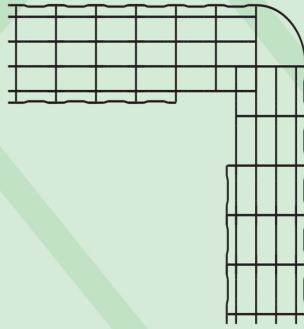
SMALL RADIUS HORIZONTAL BENDS
